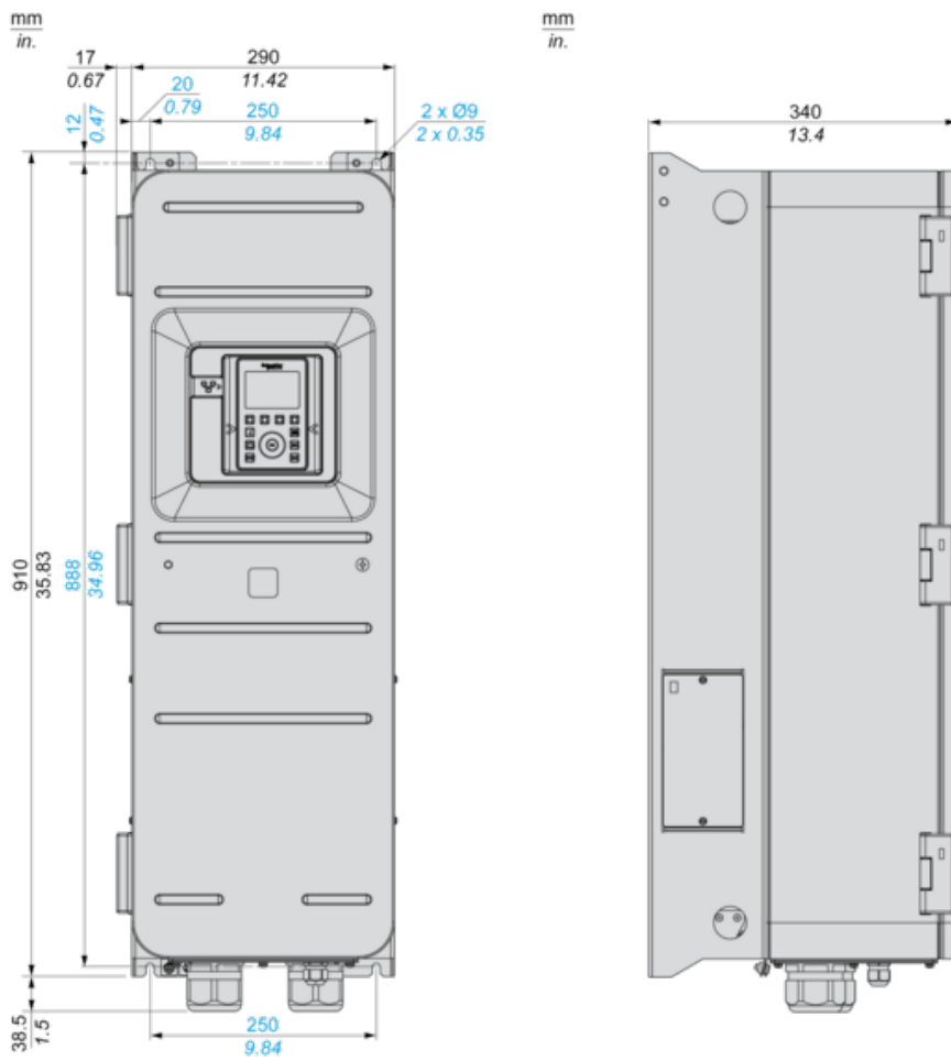
Front and Left View
